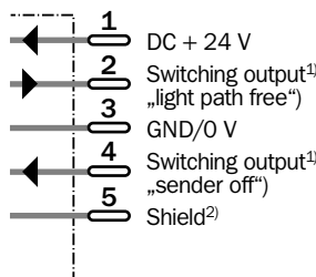
5-pin, M 12
