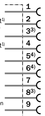
9-pin bush
