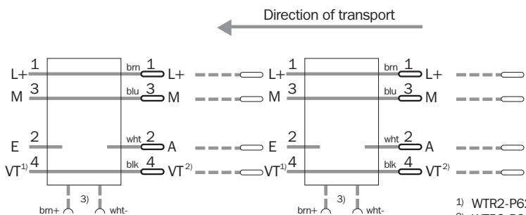
4-pin, M12
