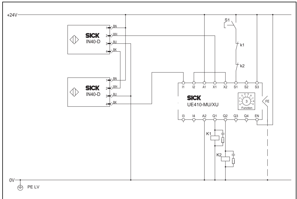
Fig. 44: Connection of two IN4000
