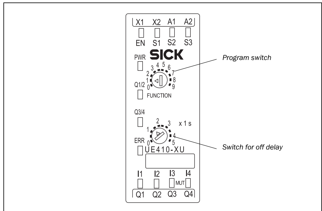
Fig. 8: UE410-XU operating and display elements
