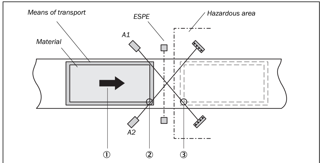
Fig. 20: Schematic layout
