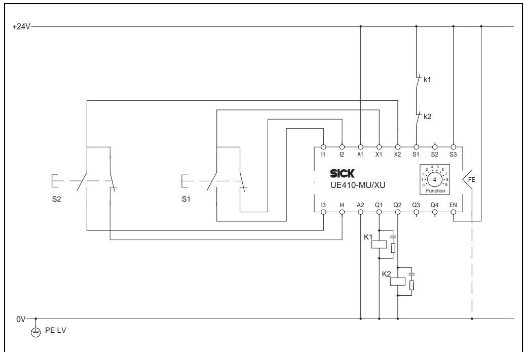
Fig. 41: Connection of a two-hand switch III C
