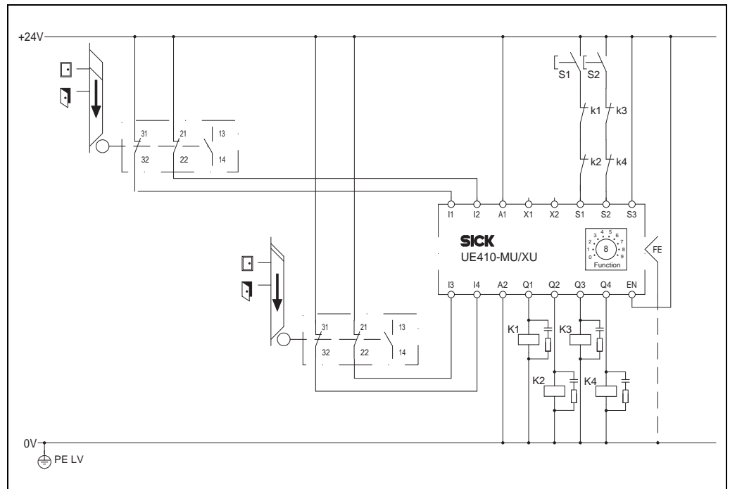
Fig. 43: Connection of two i11, two hazardous areas
