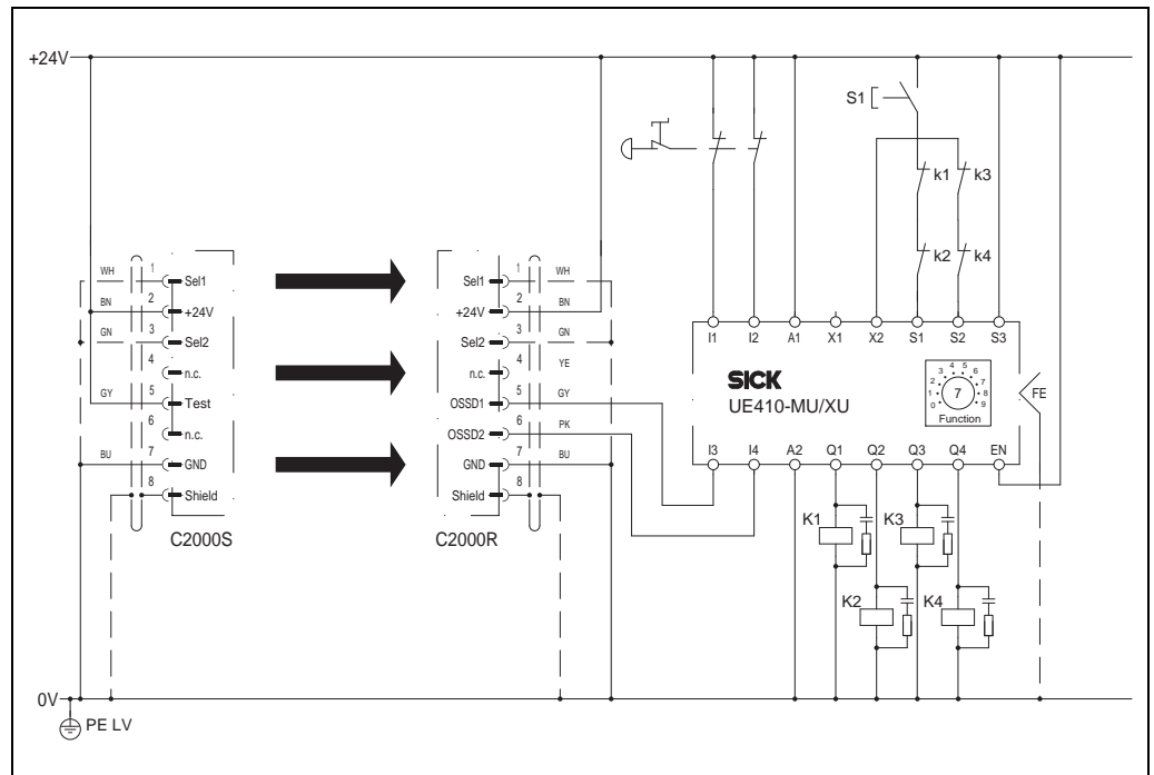
Fig. 42: Connection of a C2000 and emergency stop
