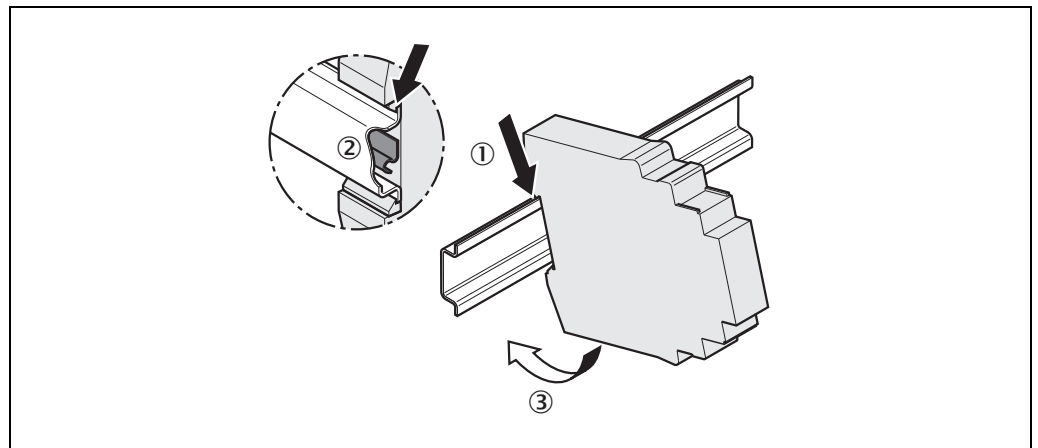
Fig. 32: Hanging the module into the DIN rail
