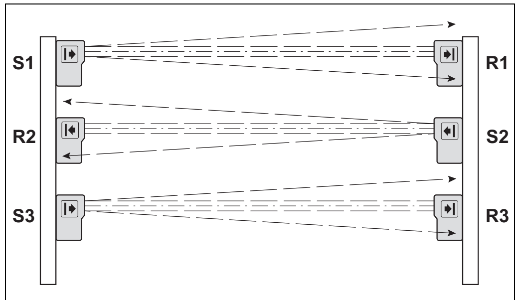
Fig. 16: Mounting to avoid mutual optical influence
