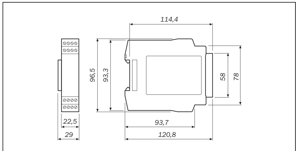
Fig. 47: Dimensional drawing UE410-XU, UE410-8DI, UE410-2RO, UE410-4RO, UE410-PRO, UE410-DEV, UE410-CAN (mm)
