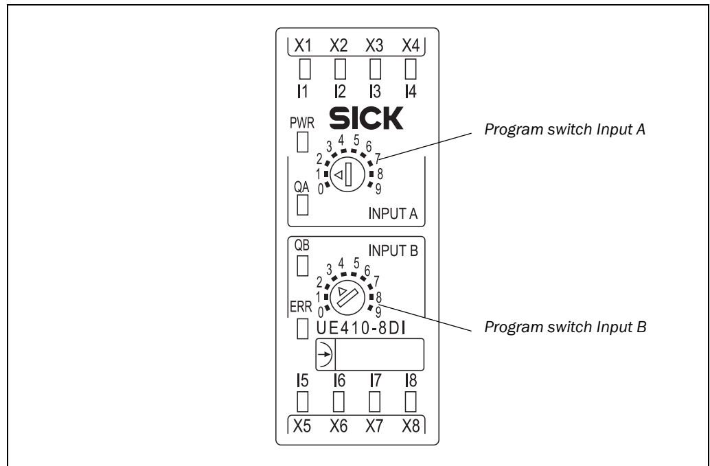
Fig. 9: UE410-8DI operating and display elements
