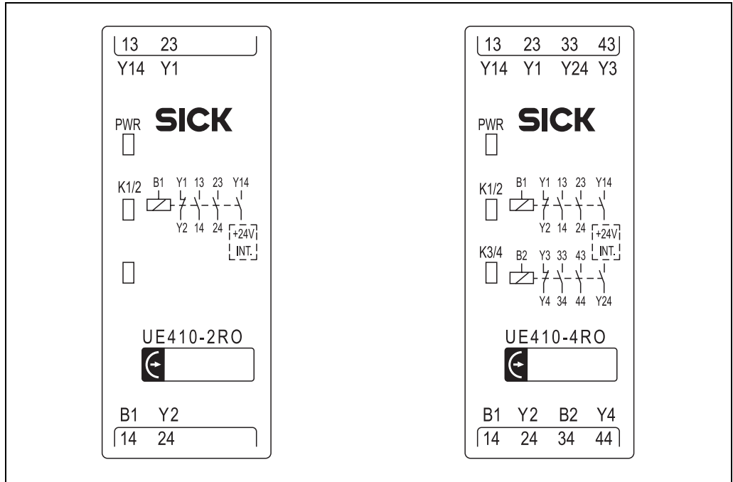
Fig. 12: Controls and status indicators UE410-2RO/UE410-4RO
