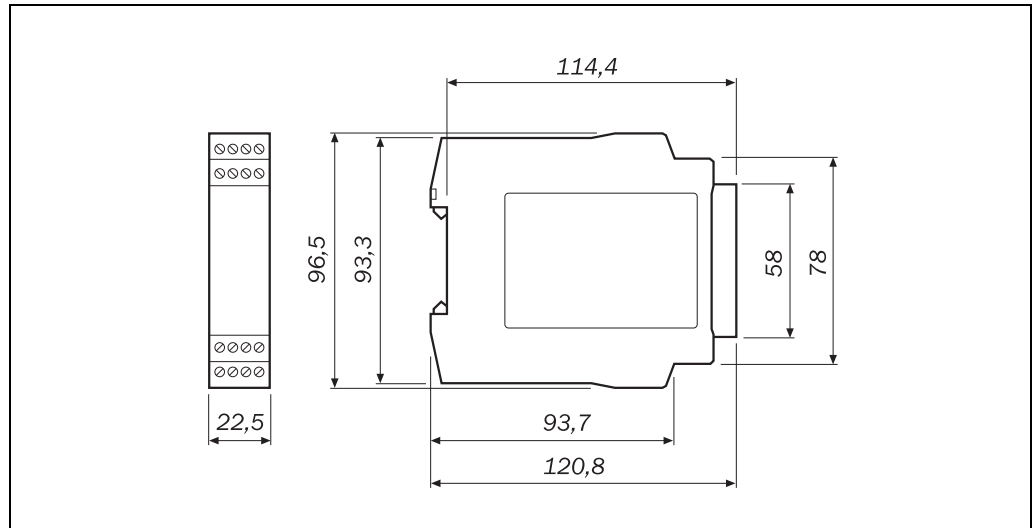
Fig. 46: Dimensional drawing UE410-MU (mm)
