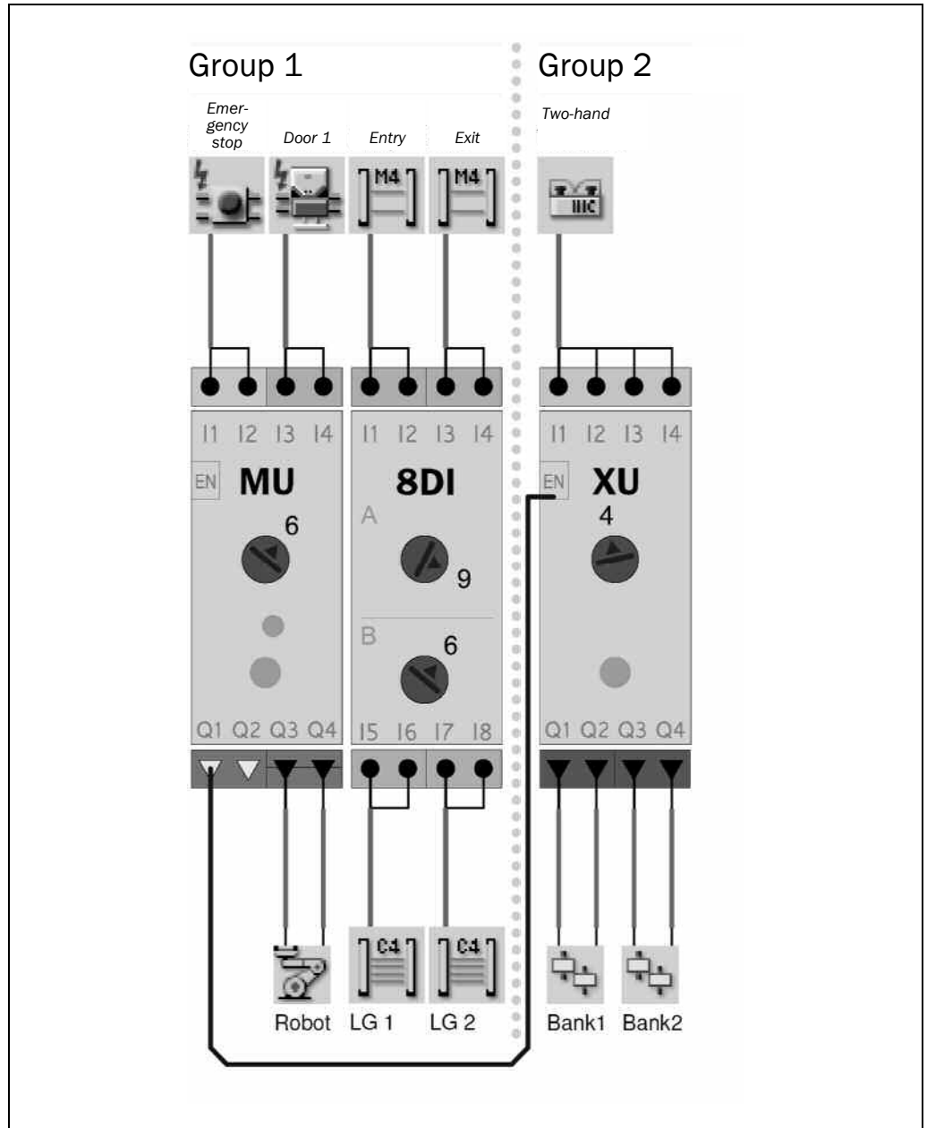
Fig. 30: Cascading of safety circuits
