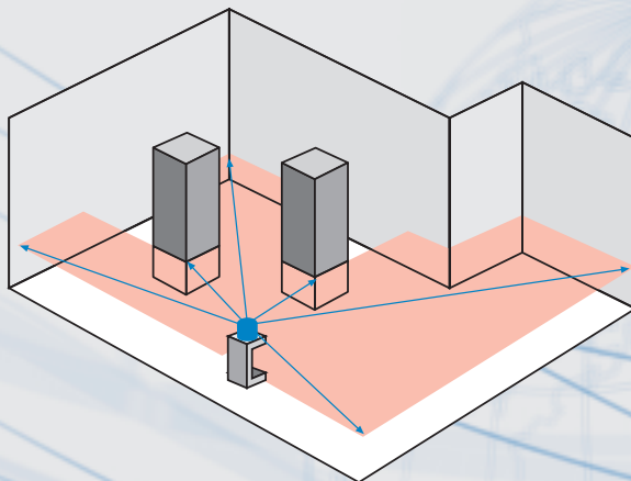
Laser scanner for surveillance of rooms
